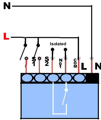
Alternative Electrical Diagram for 240V AC
