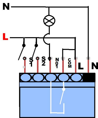
Electrical Diagram for 240V AC
